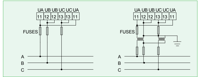
3 phase 3 wire
