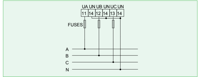
3 phase 4 wire
